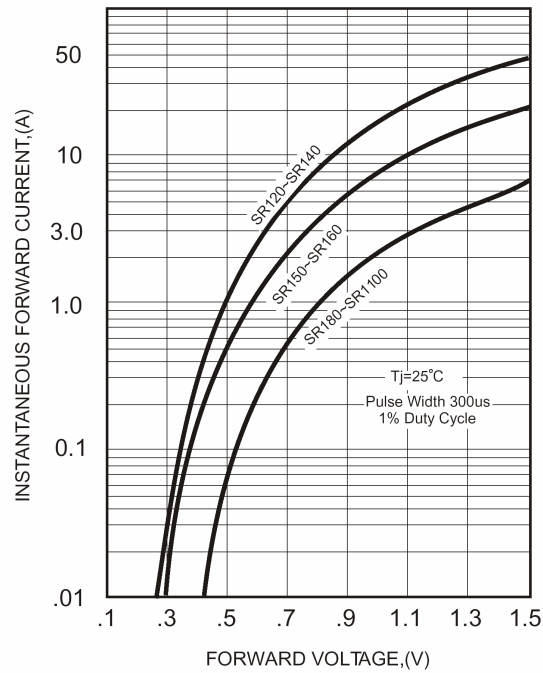
FIG.2-TYPICAL FORWARD CHARACTERISTICS
